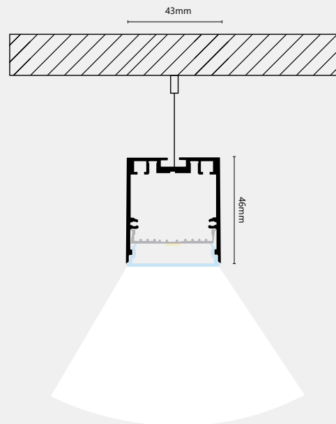
PENDEL
