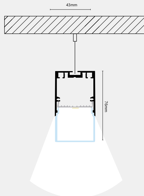
PENDEL
